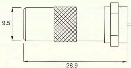
ADAPTORS Part No. EF-311A TV Male to F Male
