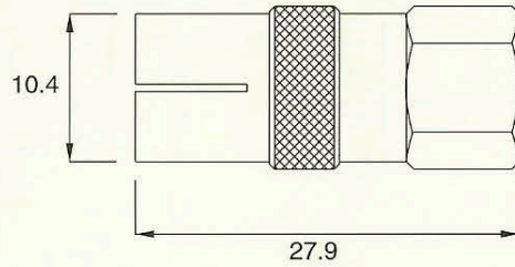
Part No. EF-321A TV Female to F Male
