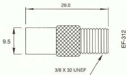
Part No. EF- 312 TV Male to F Female
