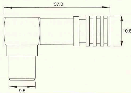
Part No. E-412BA/0.36 Male - right angle for RG6 cable
