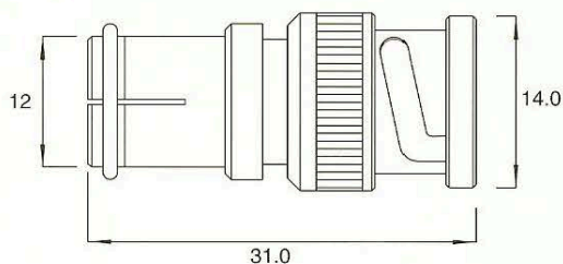
Part No. EB- 321 BNC Male to IEC Female
