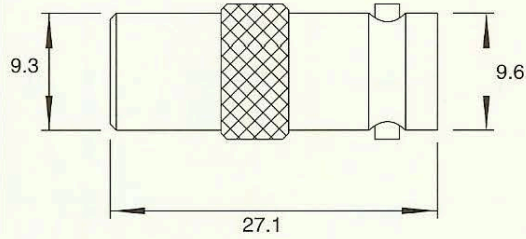
Part No. EB-312 BNC Female to TV Male
