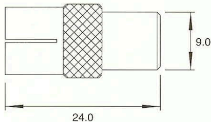
Part No. E312S-9.0 TV Male 9.0 to TV Female - European
