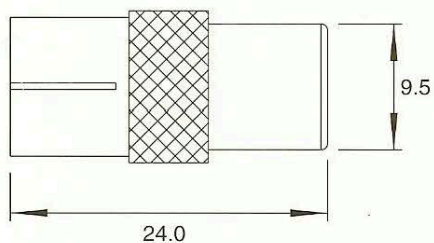
Part No. E312S TV Male 9.5 to TV Female
