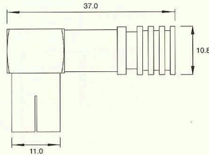
Part No. E-422BA/0.36 Female - right angle for RG6 cable
