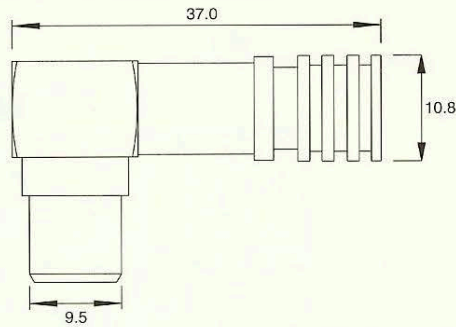
Part No. E-412BG/0.36 Male - right angle for RG59 cable
