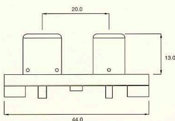
Part No. RWS-01 Edge mount, bracket assembly
