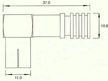
Part No. E-422BG/0.36 Female - right angle for RG59 cable
