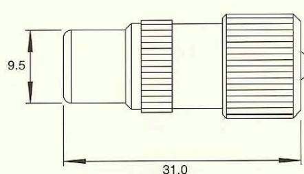
Part No. E-M112 TV Male - all metal
